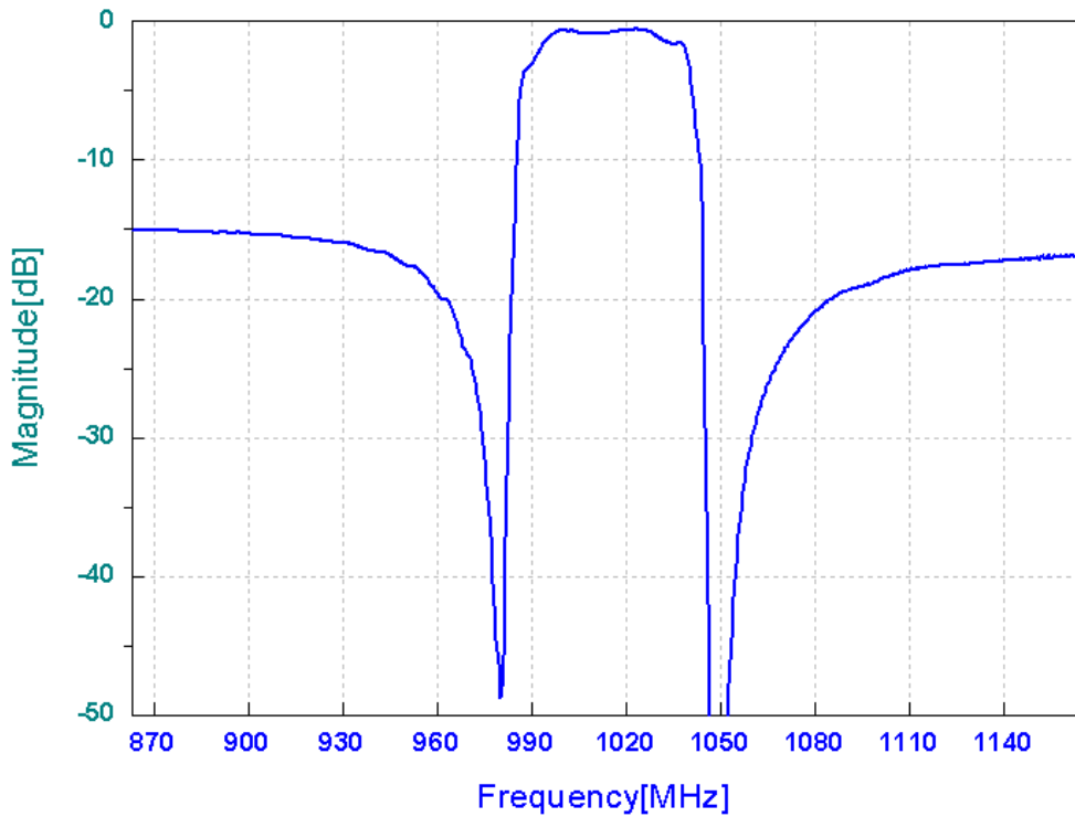
Frequency Response
